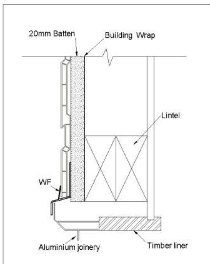
Fig 13 Window Head - Cavity Batten
