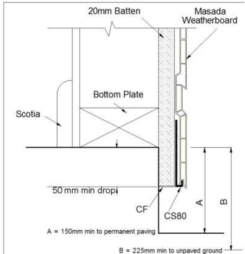
Fig 1 Bottom Wall Cavity Starter
