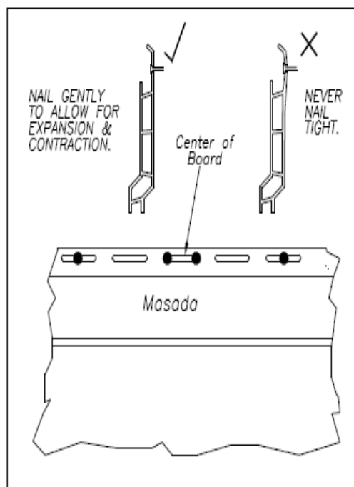
Fig 15 Fixing Details
