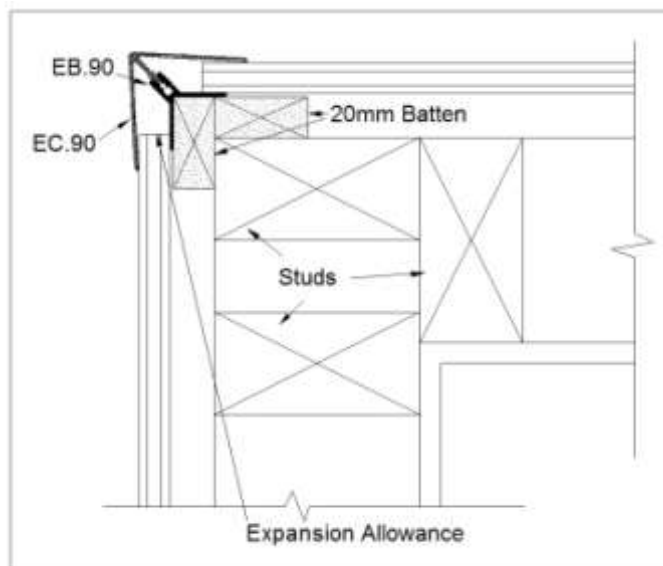
Fig 4 90° External Corner
