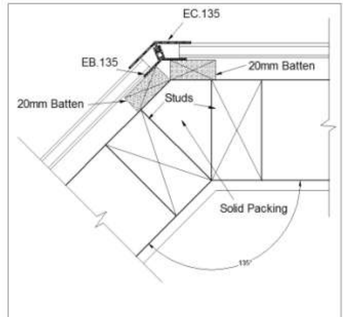
Fig 6 135° External Cavity Corner
