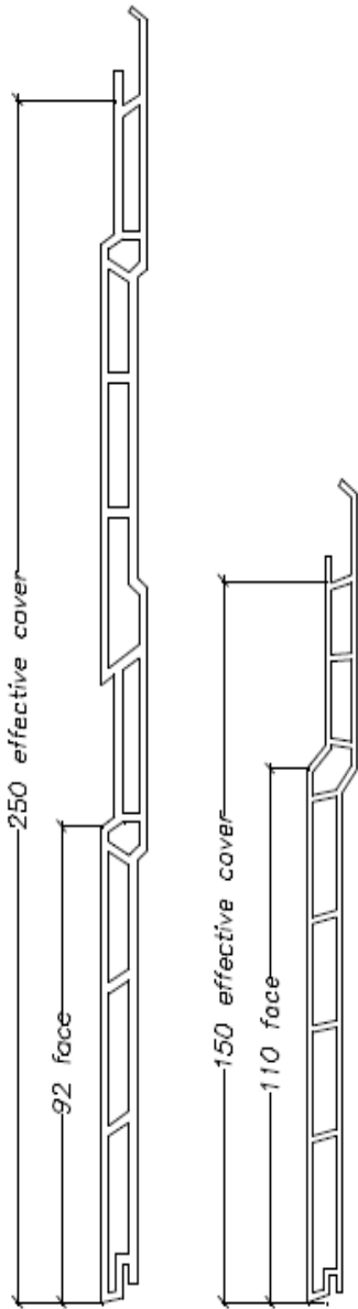
D5 & IP: 250mm & 150mm cover boards
