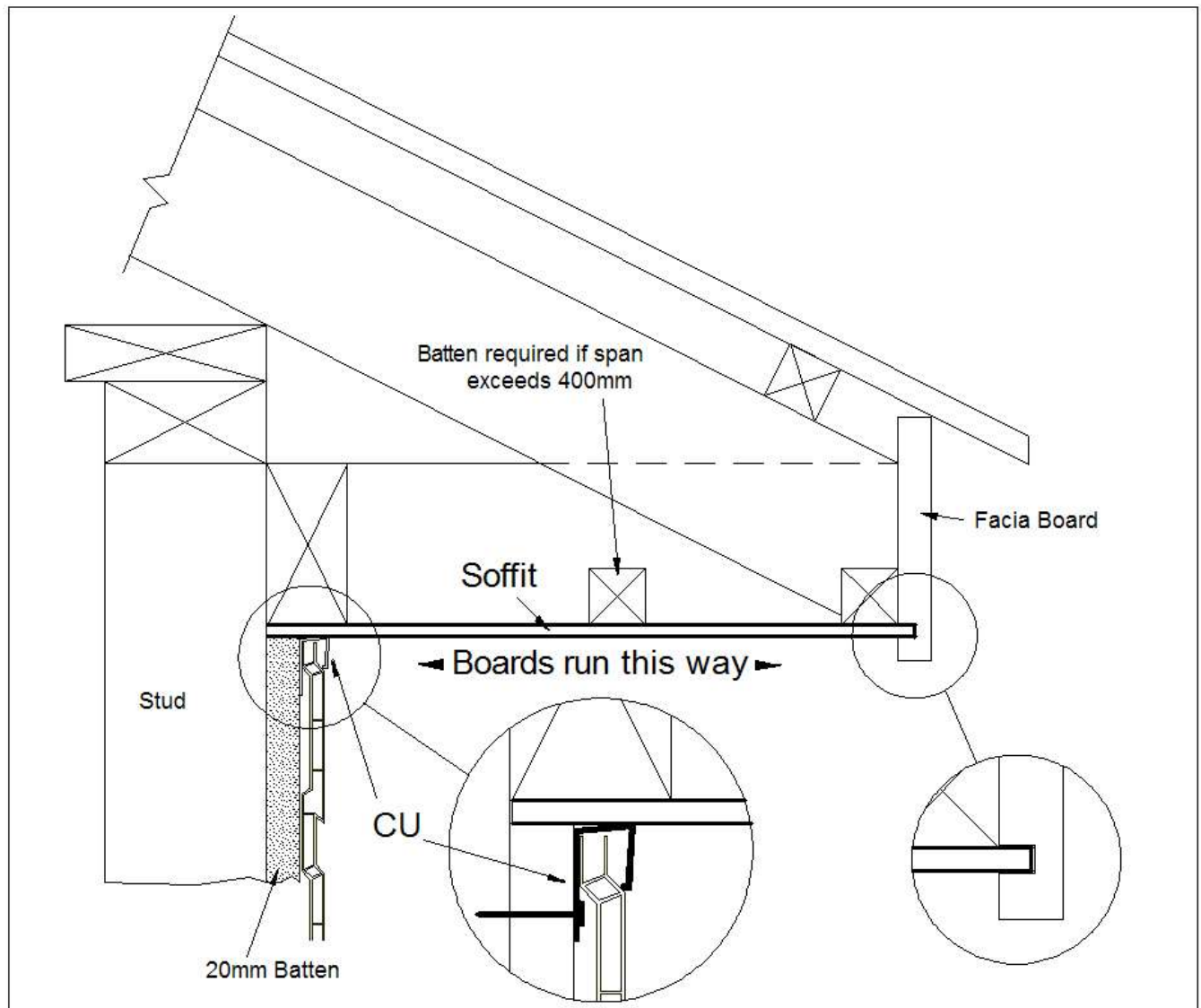
Fig 21 Soffit Detail
