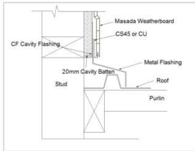
Fig 18 Roof Flashing
