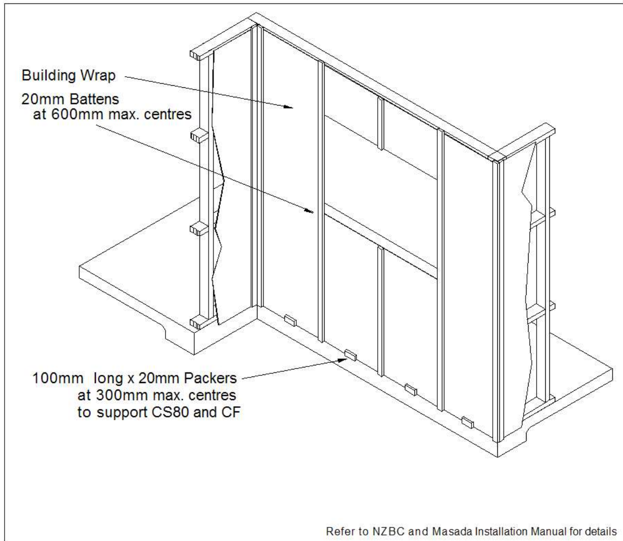
Cavity Batten Layout Diagram
