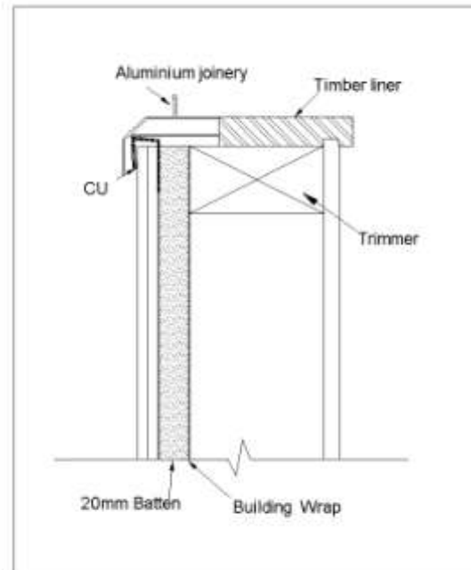
Fig 8 Window Jamb - Cavity Batten
