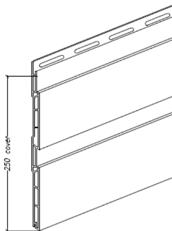
MASADA® D5 Building Board Profile
