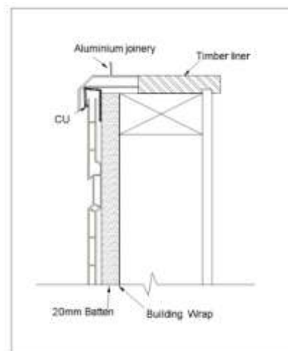
Fig 7 Window Sill - Cavity Batten
