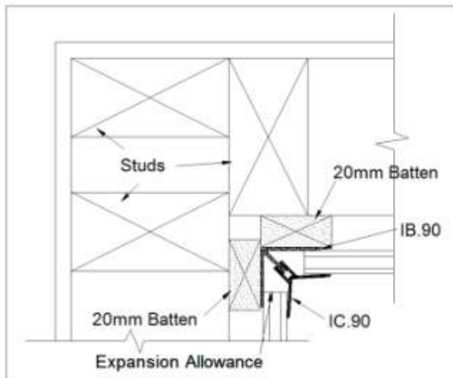
Fig 3a 90° Internal Cavity Corner
